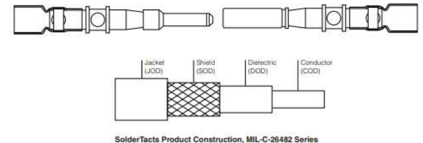
SolderTacts Product Construction, MIL-C-26482 Series
